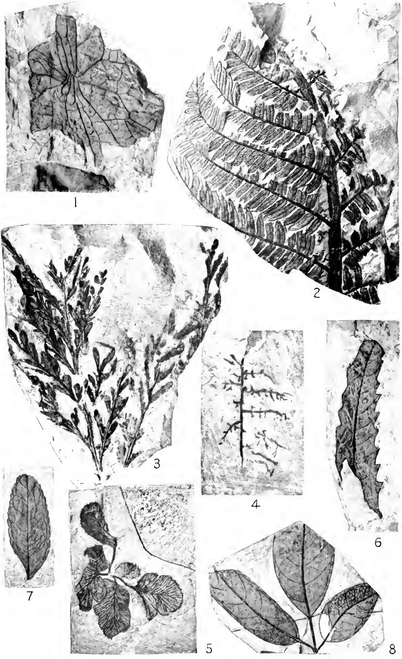
1, Nelumbo reynoldsi , new species; 2, Cladophlebis scadi , new species; 3, Anomia tremonti Knowlton; 4, Microtaenia paucifolia (Hall) Knowlton; 5, Asplenium occidentale Knowlton; 6, Degandroides lanceolata Knowlton; 7, Sapindopsis schultzi , new species; 8, Staphylea? tremonti Knowlton. All natural size
